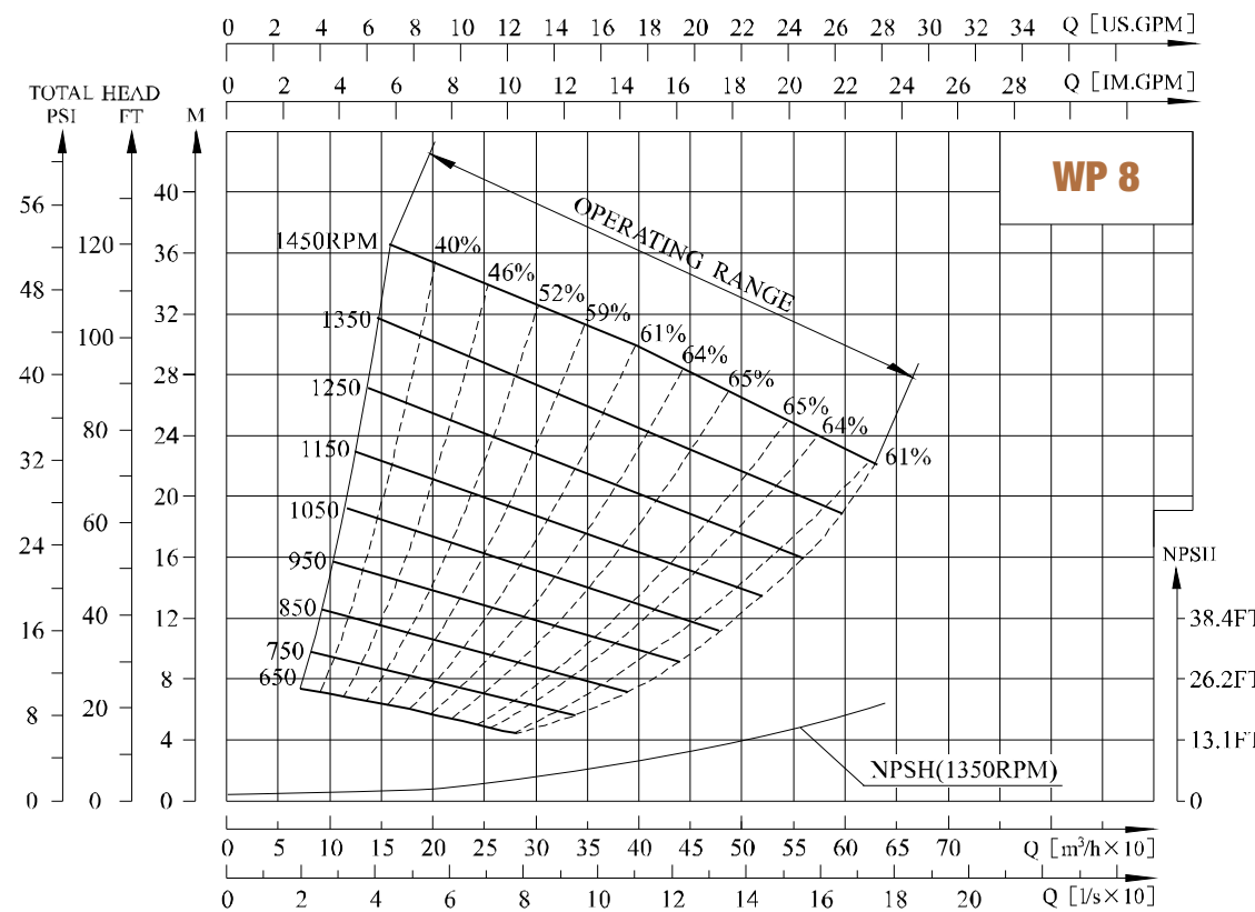
Performance curve
