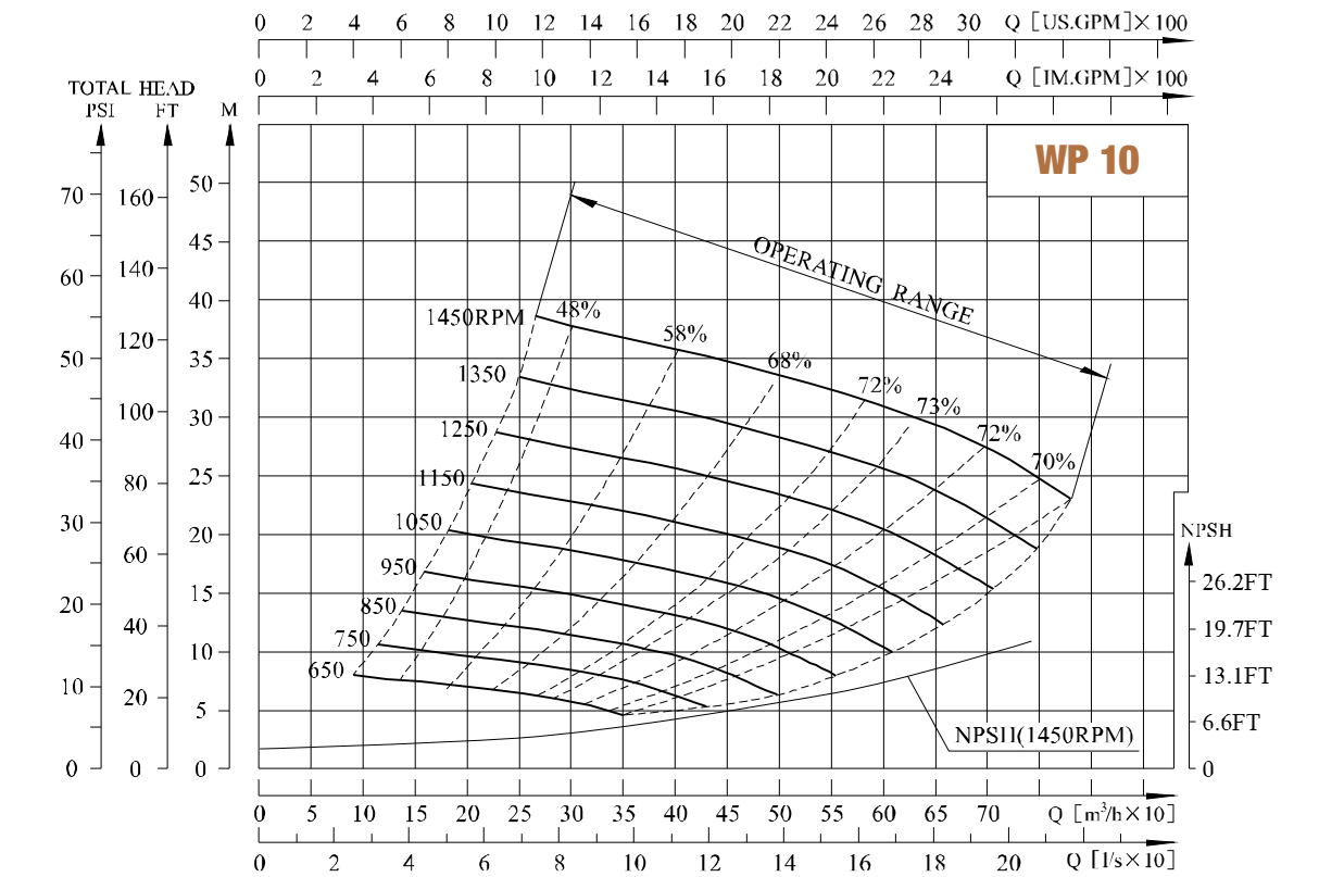
Performance curve
