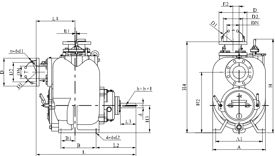
Pump profile and installation dimension
